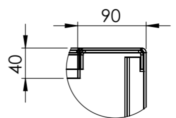
DETAIL B SCALE 1 : 5
